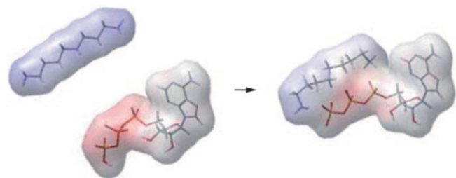
Figure 1. Hypothetical images of the SPD–ATP complex. The molecular surface is colored to indicate atom charges. The conformation of the complex on the right is that shown in Figure 4c.
