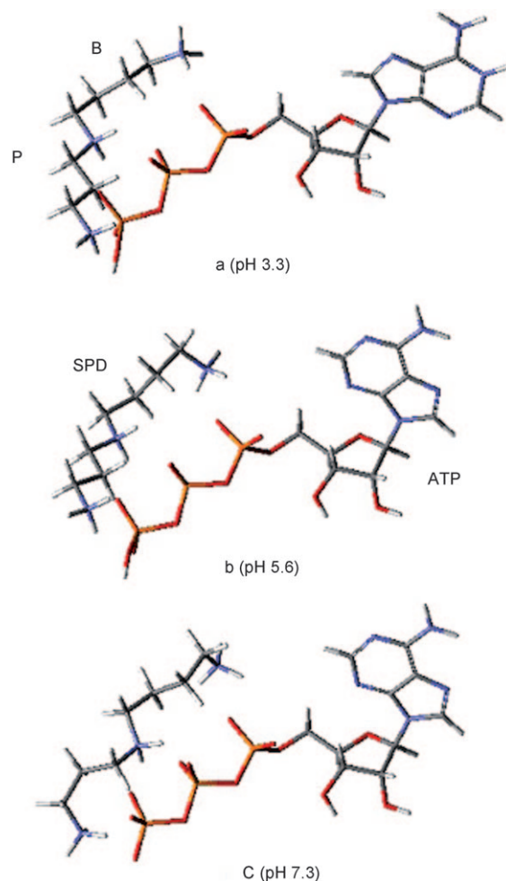
Figure 4. Hypothetical images of the SPD shapes accounting for the pH-dependent increase in gauche orientation. Three of the many possible conformations, a–c, are depicted. The orientations of the C2–C3, C3–C4, C4–N5, N5–C6, C6–C7, C7–C8, and C8–C9 bonds are AAGAAAA in (a), GAGAAAA in (b), and GAGAG'AG in (c). The conformation of ATP was obtained by calculations with the OPLS force field. When the pH value was raised from 3.3, the orientation of the adenine group of ATP switches to the syn conformation at pH 5.6, which leads to the bent butylene part (B). The conformation of the propylene part (P) is further altered by the second deprotonation of the \gamma -phosphate group at pH 7.3. The relative positioning of SPD and ATP derived from the simulation is not based on experimental data.
