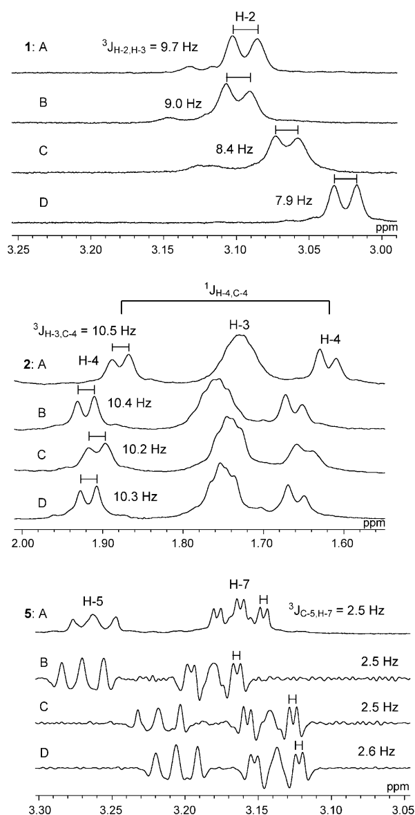
Figure 2. Partial ^1\text{H} NMR spectra (500 MHz, 40^\circ\text{C} ) of the labeled SPDs 1 , 2 , and 5 . NMR spectra were measured with 25 mm labeled SPD as the 3HCl salt in \text{D}_2\text{O} at pH 7.3 (A), and in the presence of 100 mM ATP at pH 3.3 (B), 100 mM ATP at pH 5.6 (C), and 100 mM ATP at pH 7.3 (D). The spectra of 1–7 as the 3HCl salt at pH 3.3 and 5.6 were virtually identical with those shown in (A). Resolution enhancement was carried out for the spectra of compounds 4 and 5 in the presence of ATP. The spectra of other labeled SPDs are provided in the Supporting Information.
